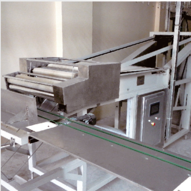
Rotary Cutting Machine 旋转式切断机
