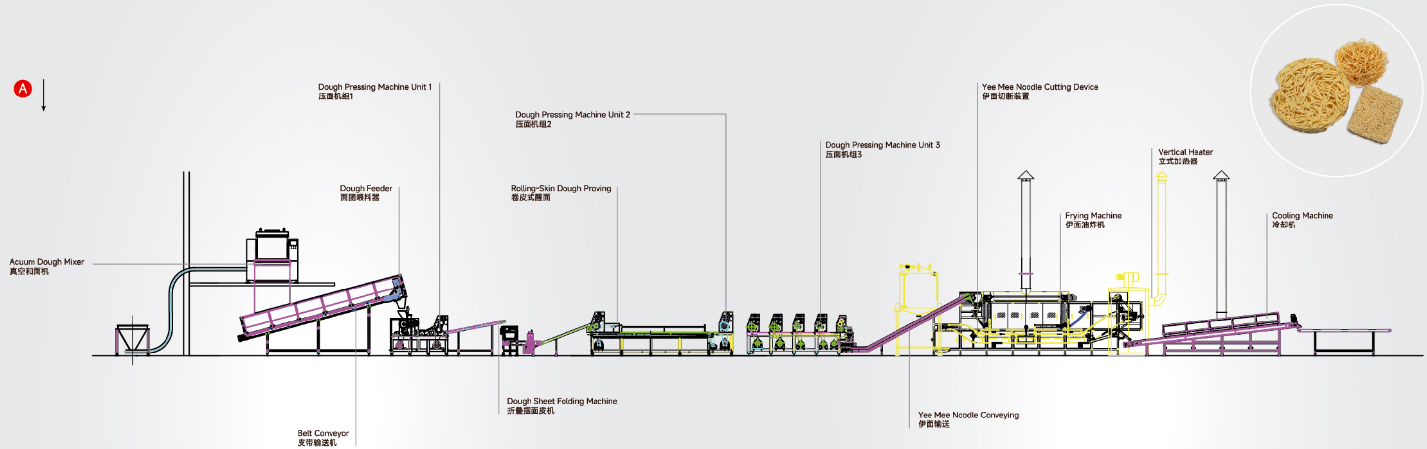
Flow Chart of Raw Fried Yee Mee (Crispy Noodles) Production Line
