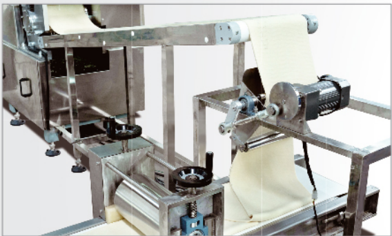
◆ Dough Sheet Cross-layering Machine 交叉叠皮机
