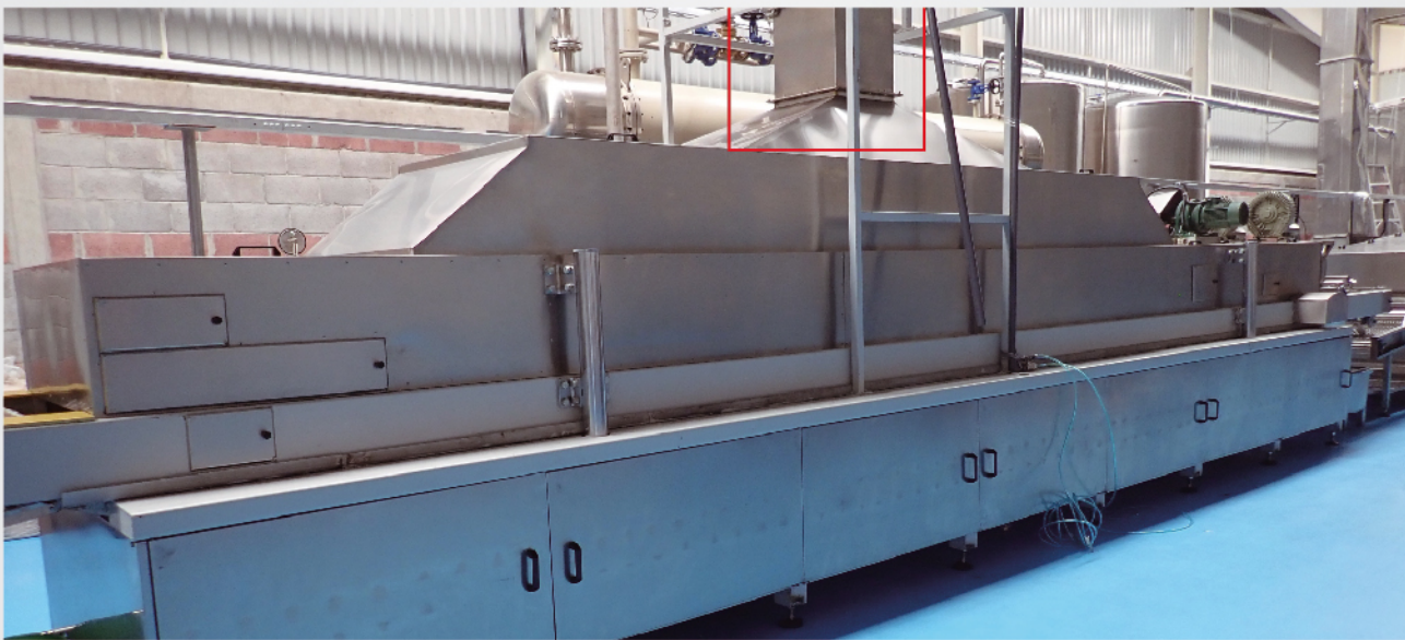
Automatic Frying Machine 油炸机
